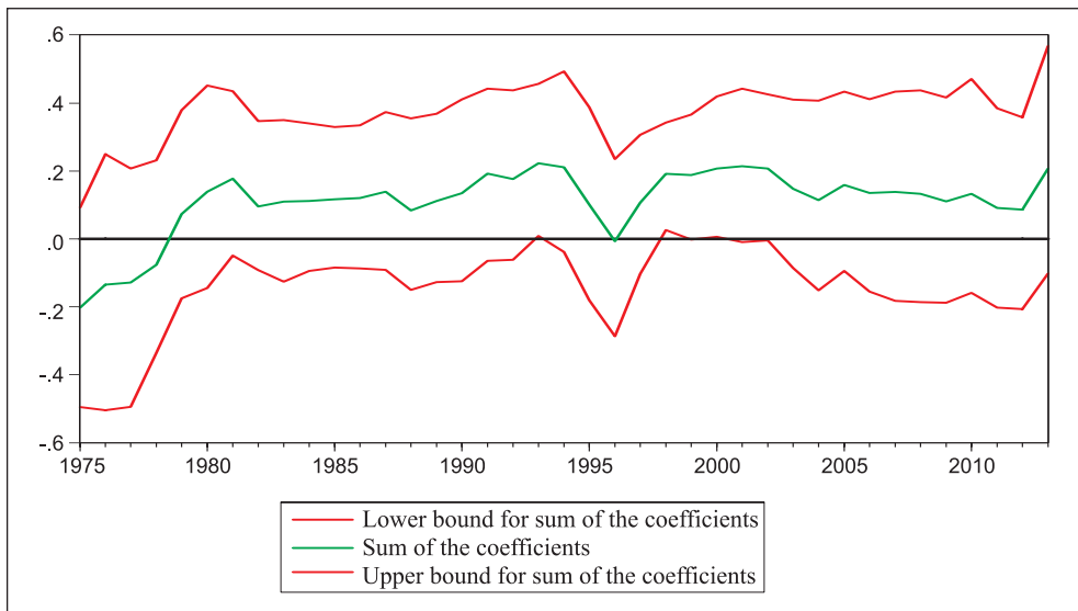
Figure 3: Bootstrap estimate of the sum of the rolling coefficients for the impact of LNPSG on LNCGDP
